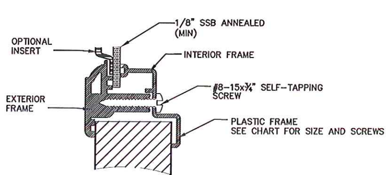
DETAIL I NON-IMPACT GLAZING
