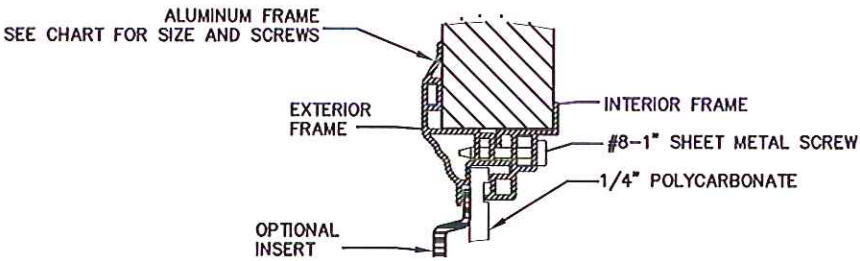
DETAIL K IMPACT GLAZING
